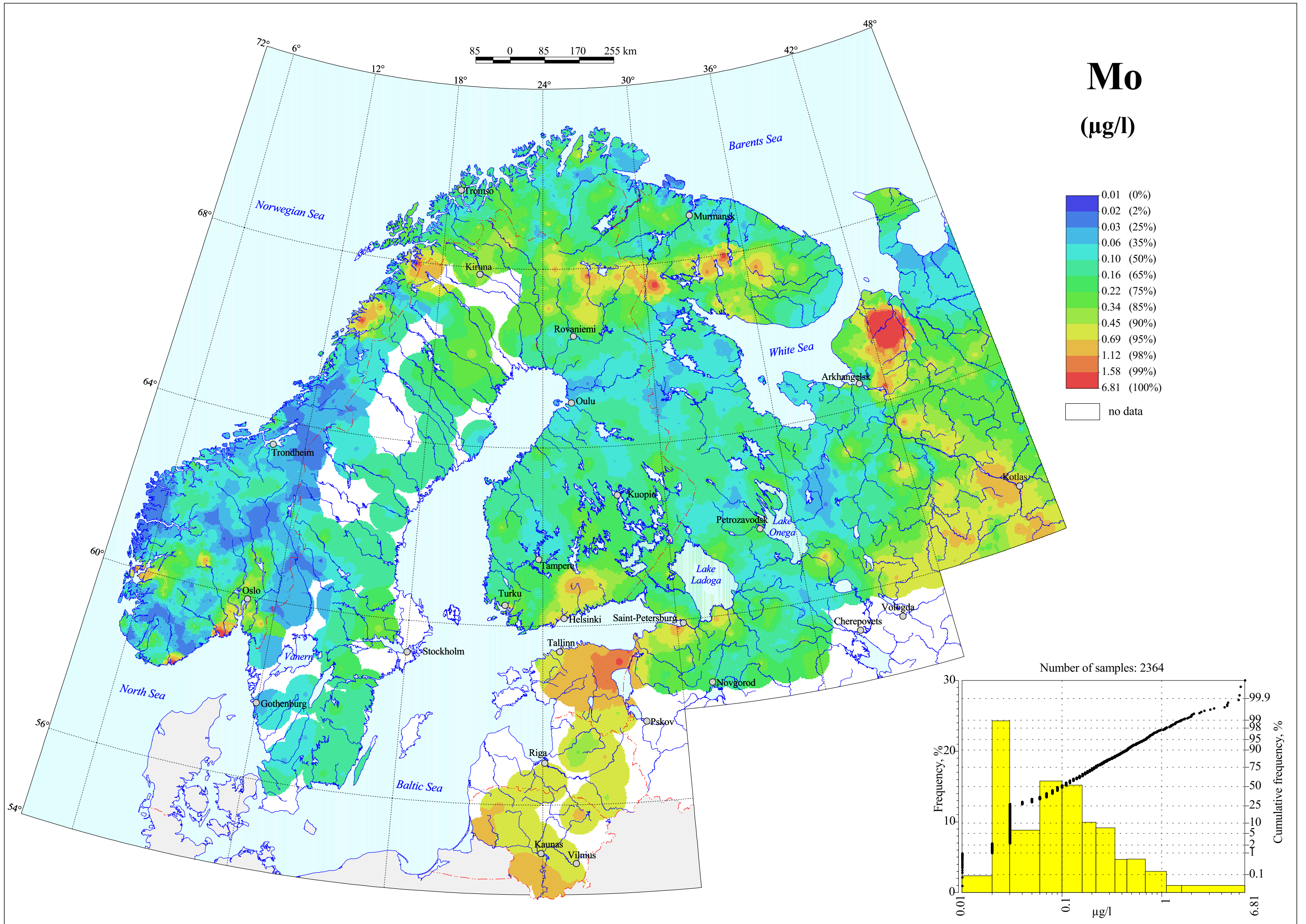
Molybdenum in Surface Water
